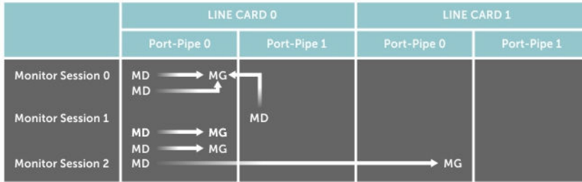
Figure 94. Port Monitoring Configurations on the S-Series
